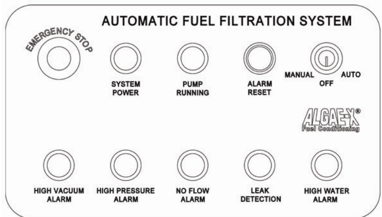
Control Panel of STS 6000-4GPM-S (with Separ option)
